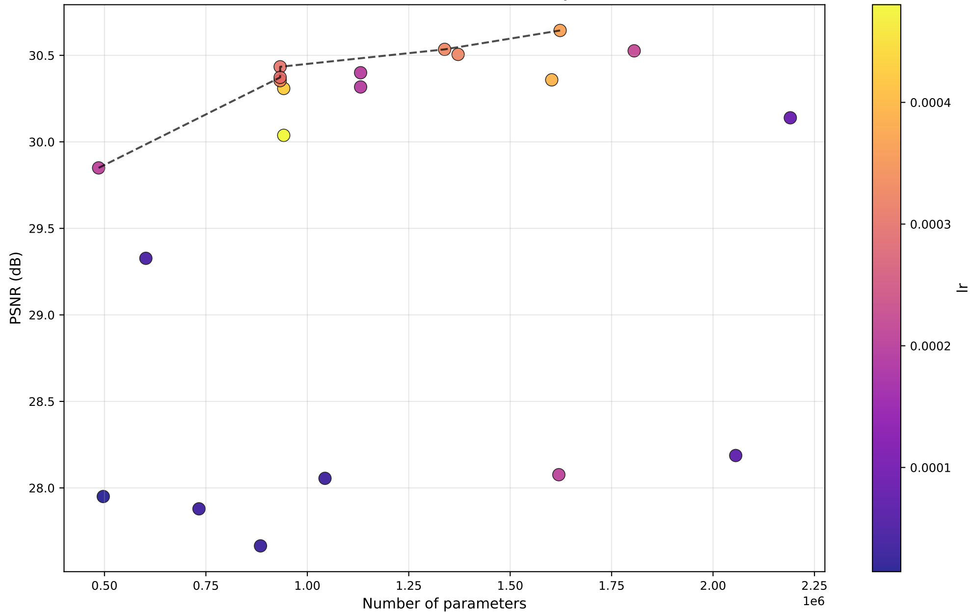
PSNR vs #Params — ELAN — by lr
